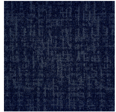
Cobalt
